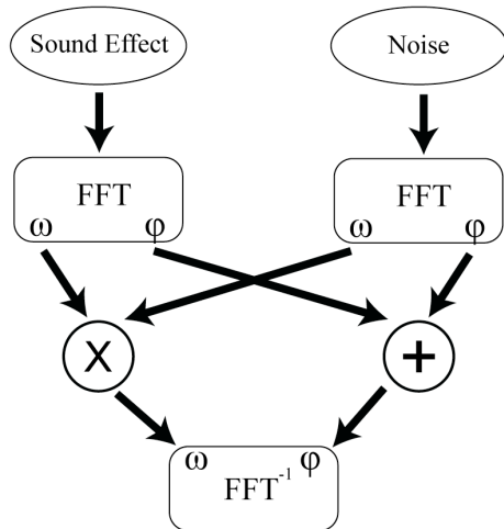
Figure 2: Cross synthesis signal flow
