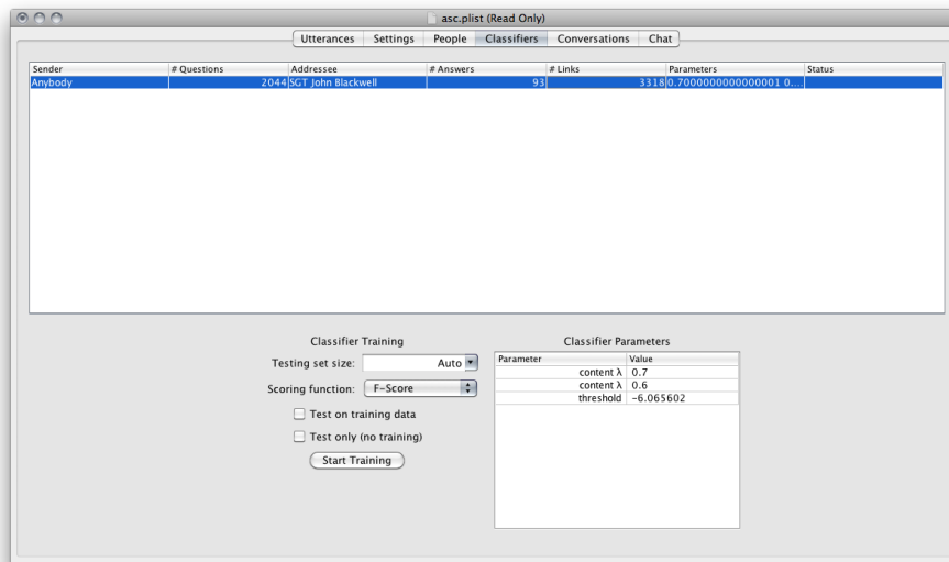
Figure 5: The classifier panel lists existing text classifiers, provides controls for classifier training, and allows an advanced user to modify the classifier parameters.
