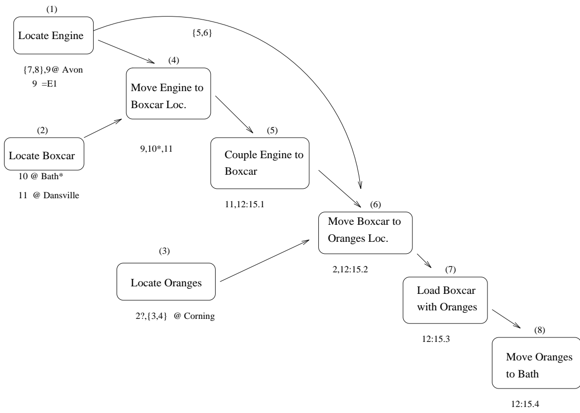
Figure 8: Domain Plan for Moving Oranges to Bath
